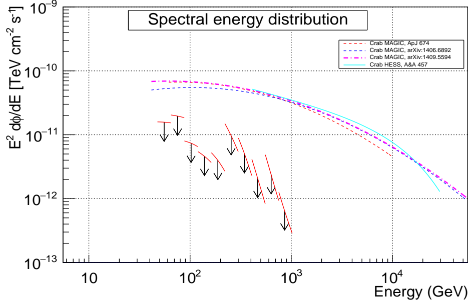
Figure 35: SED
